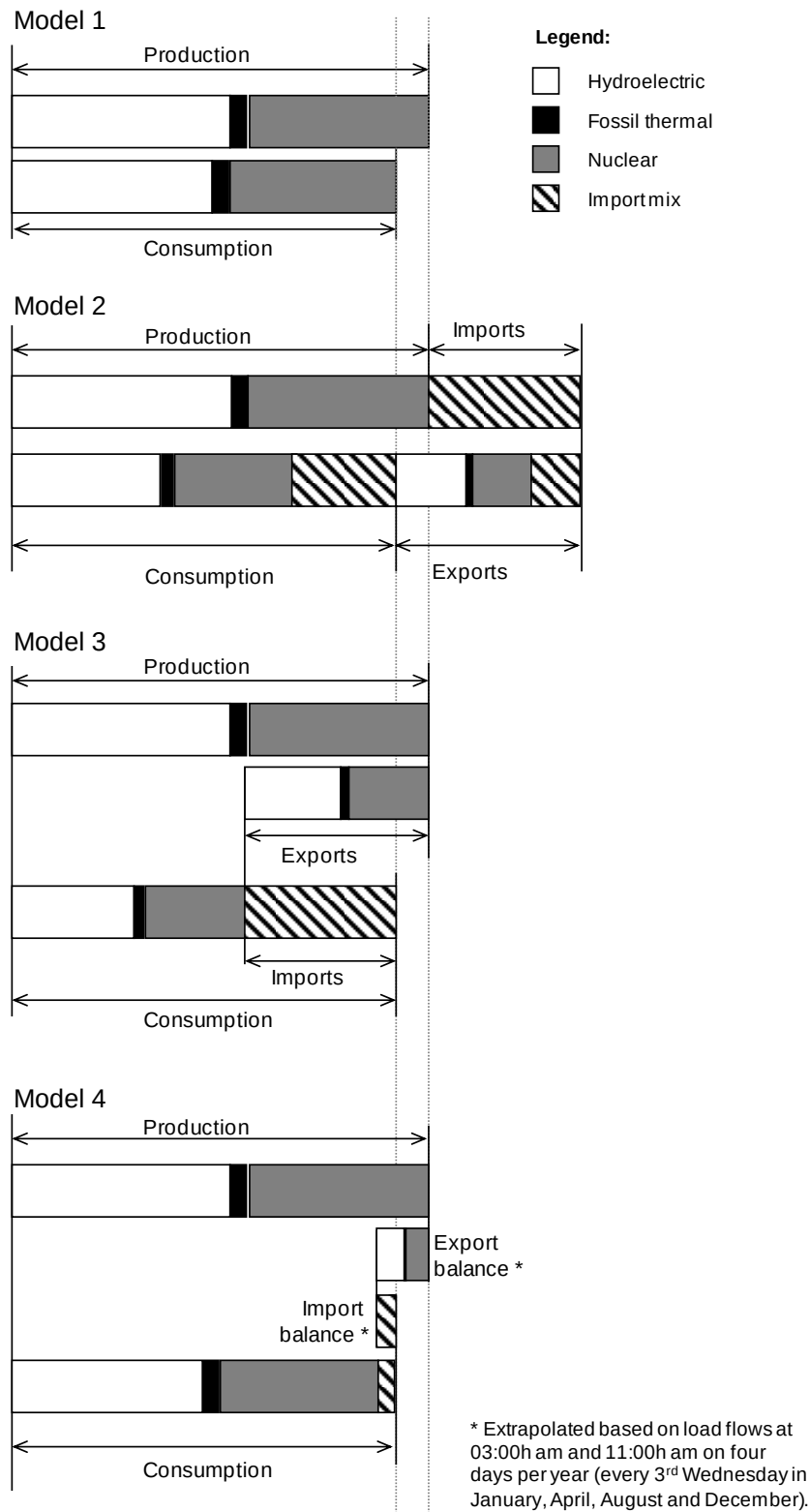
Fig. 2.1: Model approaches for electricity mixes in LCA; graphs represent annual averages (Ménard et al. 1998, S. 10-11)
